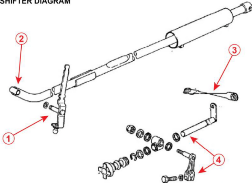
SHIFTER DIAGRAM
